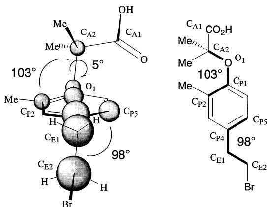
Figure 2. Structure of 2-[4-(2-bromoethyl)-2-methylphenoxy]-2-methylpropionic acid (right), the hydrolysed derivative of 3c , and its conformer at the global minimum (left).
