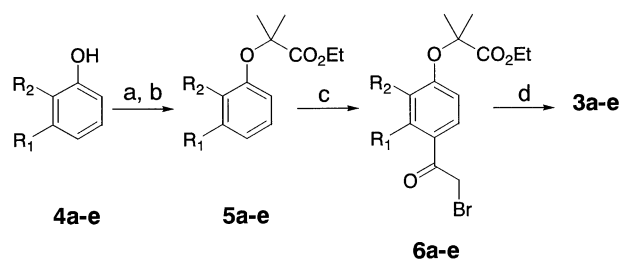
Scheme 1. General synthesis of intermediates 3 . Reagents: (a) Chloretone, NaOH; (b) SOCl_2 , EtOH; (c) bromoacetyl bromide, AlCl_3 ; (d) Et_3SiH , TFA.
