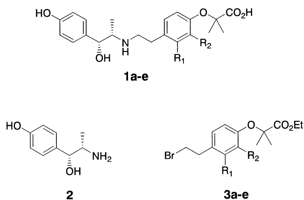
Figure 1. General formula of 2-phenoxyisobutyric acids ( 1 ) as a novel \beta_3 -adrenoceptor agonist and synthetic intermediates.
