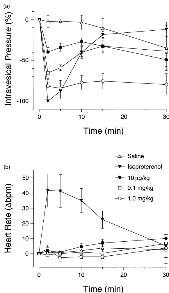
Figure 3. Time course of changes in intravesical pressure (a) and heart rate (b) in anaesthetized rats after administration of iv saline (1 mL/kg), isoproterenol (10 µg/kg), and 1a (10 µg, 0.1 mg, 1.0 mg/kg) ( n = 3 ). Intravesical pressure (a) is expressed as a percentage of the maximal relaxation with isoproterenol at 2 min. Heart rate (b) is expressed as the difference from the value before drug administration.
